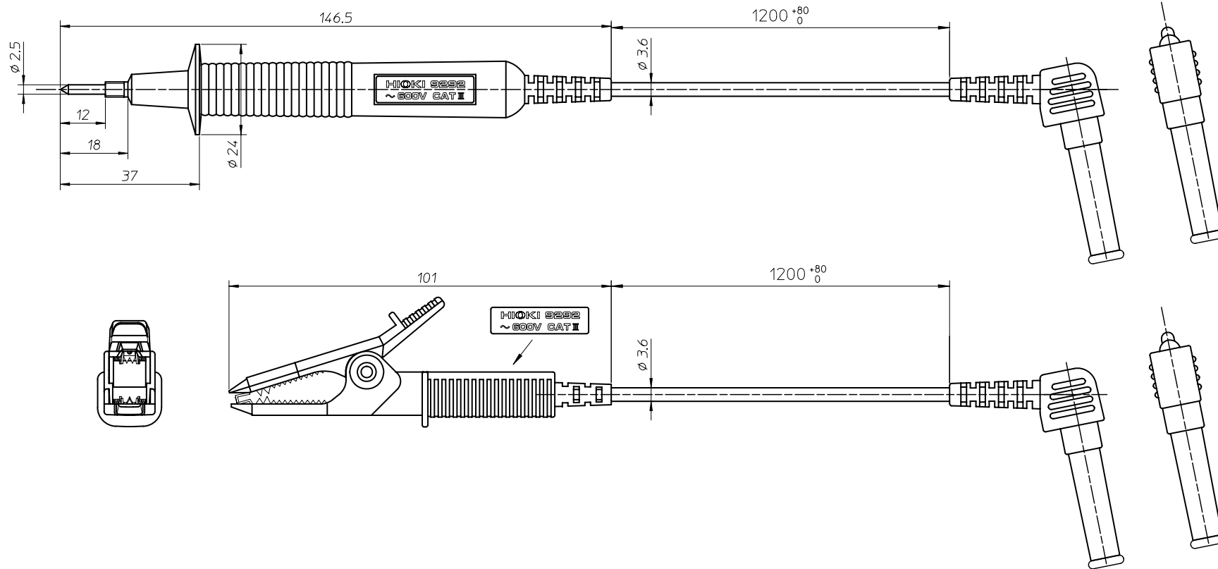
LINE_PROBE(RED)、EARTH_PROBE(BLACK) SET
